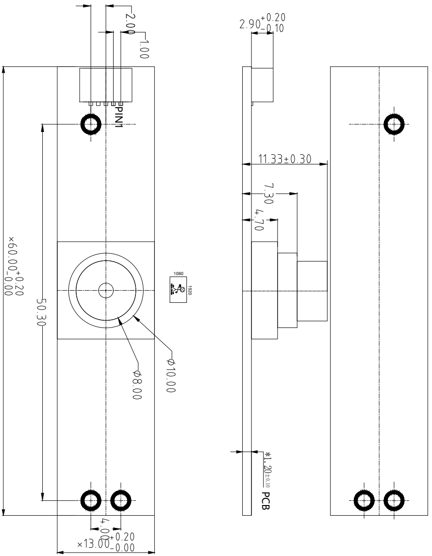
BOTTOM VIEW
